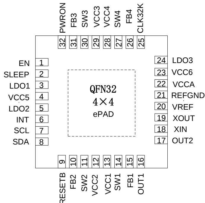
Fig. 2-2 Pin Assignment
